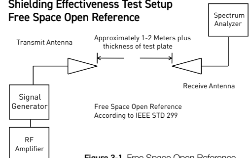
Figure 3-1. Free Space Open Reference
