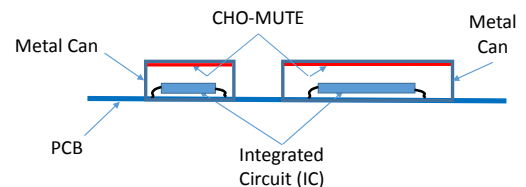
Figure 8-1 Cavity Resonance Absorber Used Inside a Metal Can
